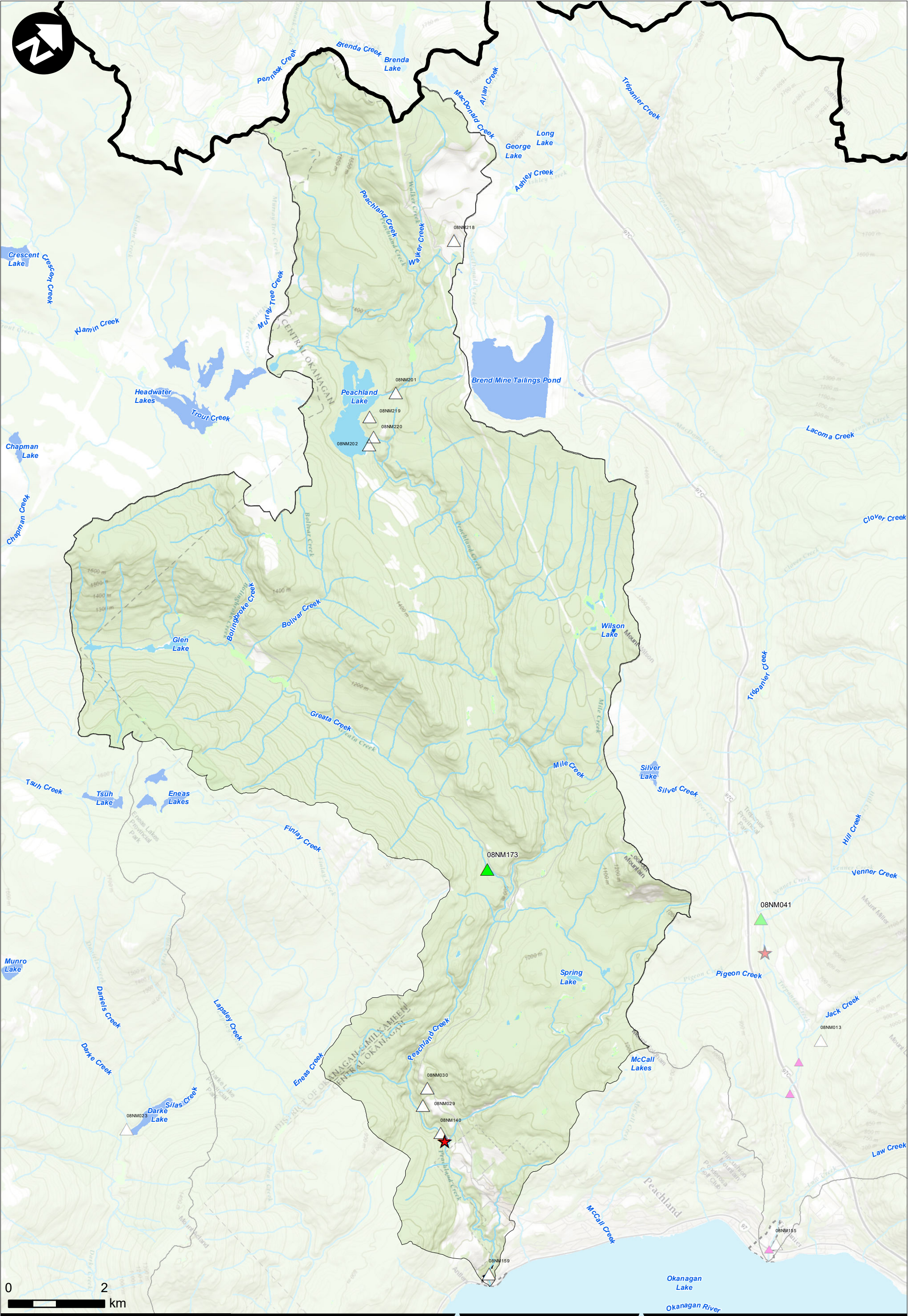
FIGURE 3-2: PEACHLAND CREEK WATERSHED OVERVIEW RDCO Peachland and Trepanier Creeks Flood Mapping
