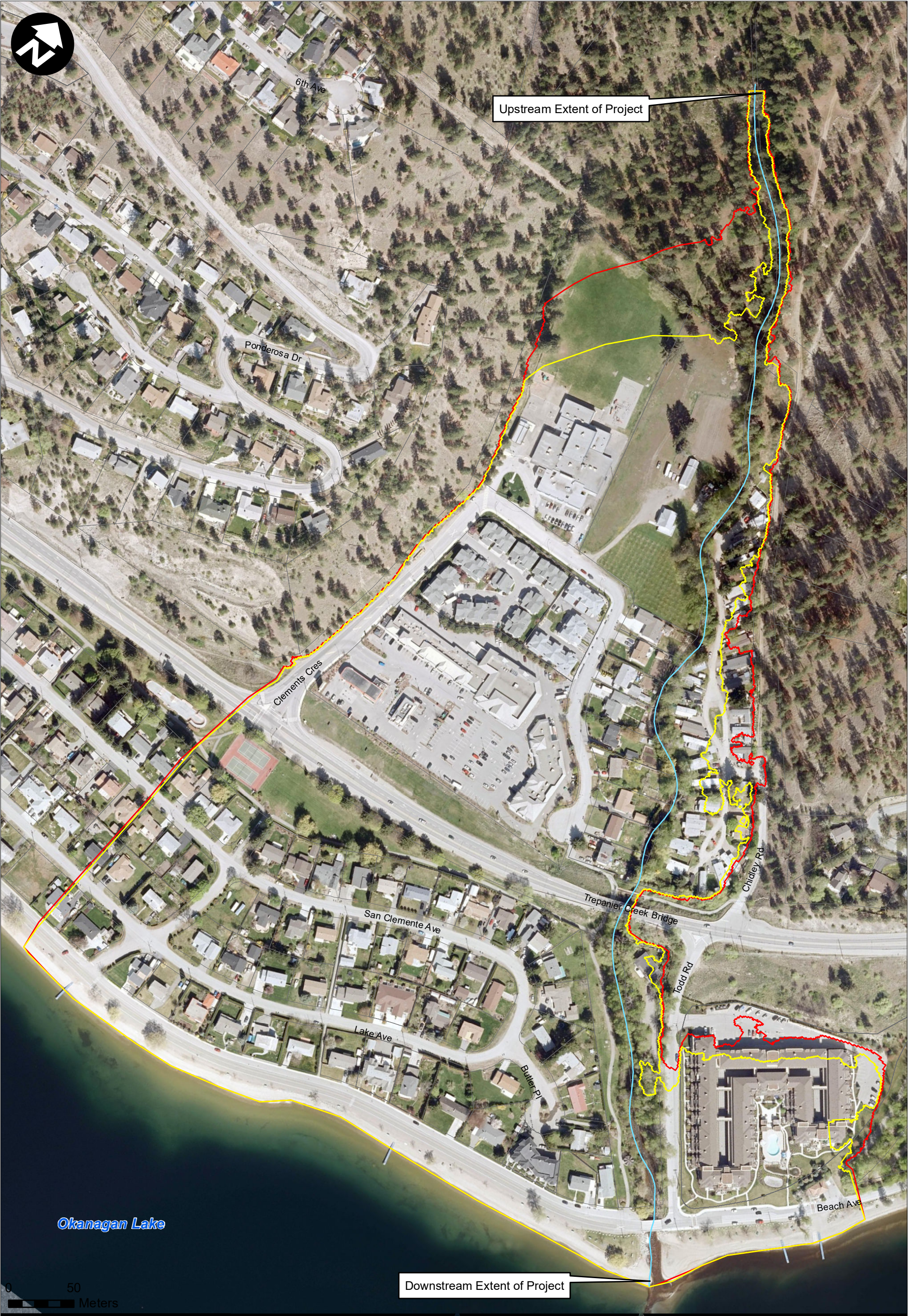
FIGURE 5-8: TREPANIER CREEK REACH 2, 200-YEAR - MINIMUM AND ADDITIONAL FREEBOARD
