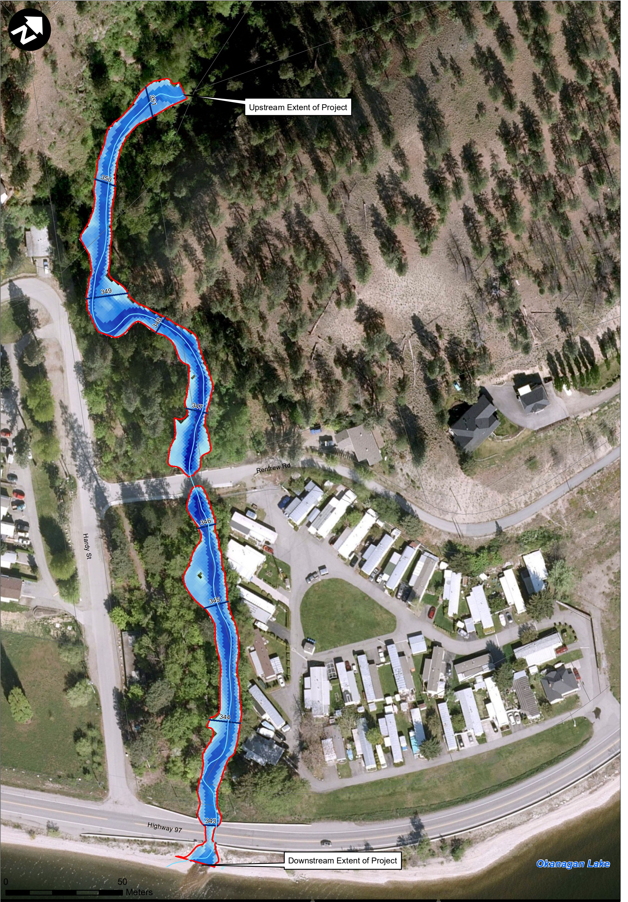
FIGURE 5-1: PEACHLAND CREEK REACH 1, 20-YEAR - NO FREEBOARD RD CO Peachland and Trepanier Creeks Flood Mapping
