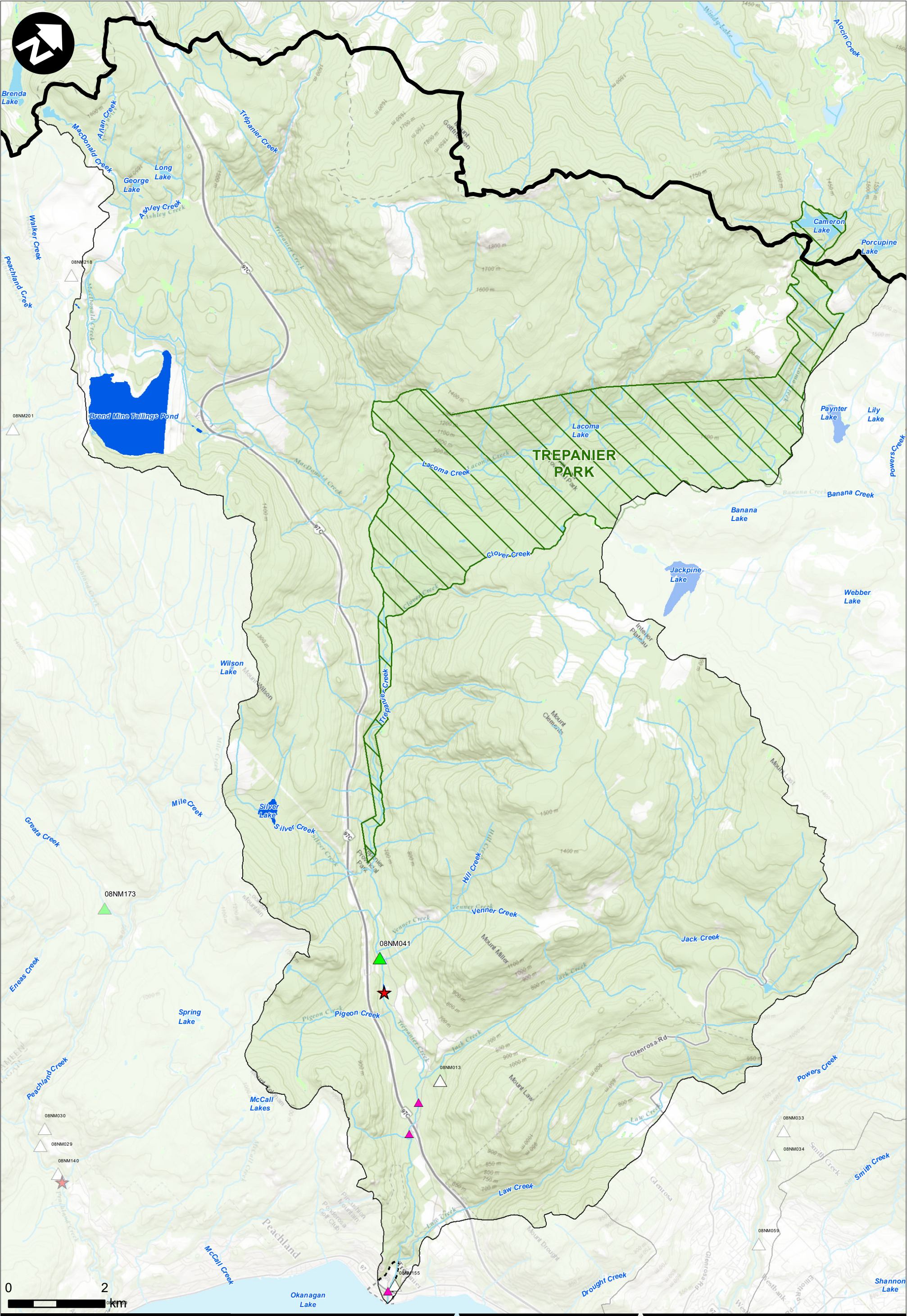
FIGURE 3-3: TREPANIER CREEK WATERSHED OVERVIEW RDCO Peachland and Trepanier Creeks Flood Mapping
