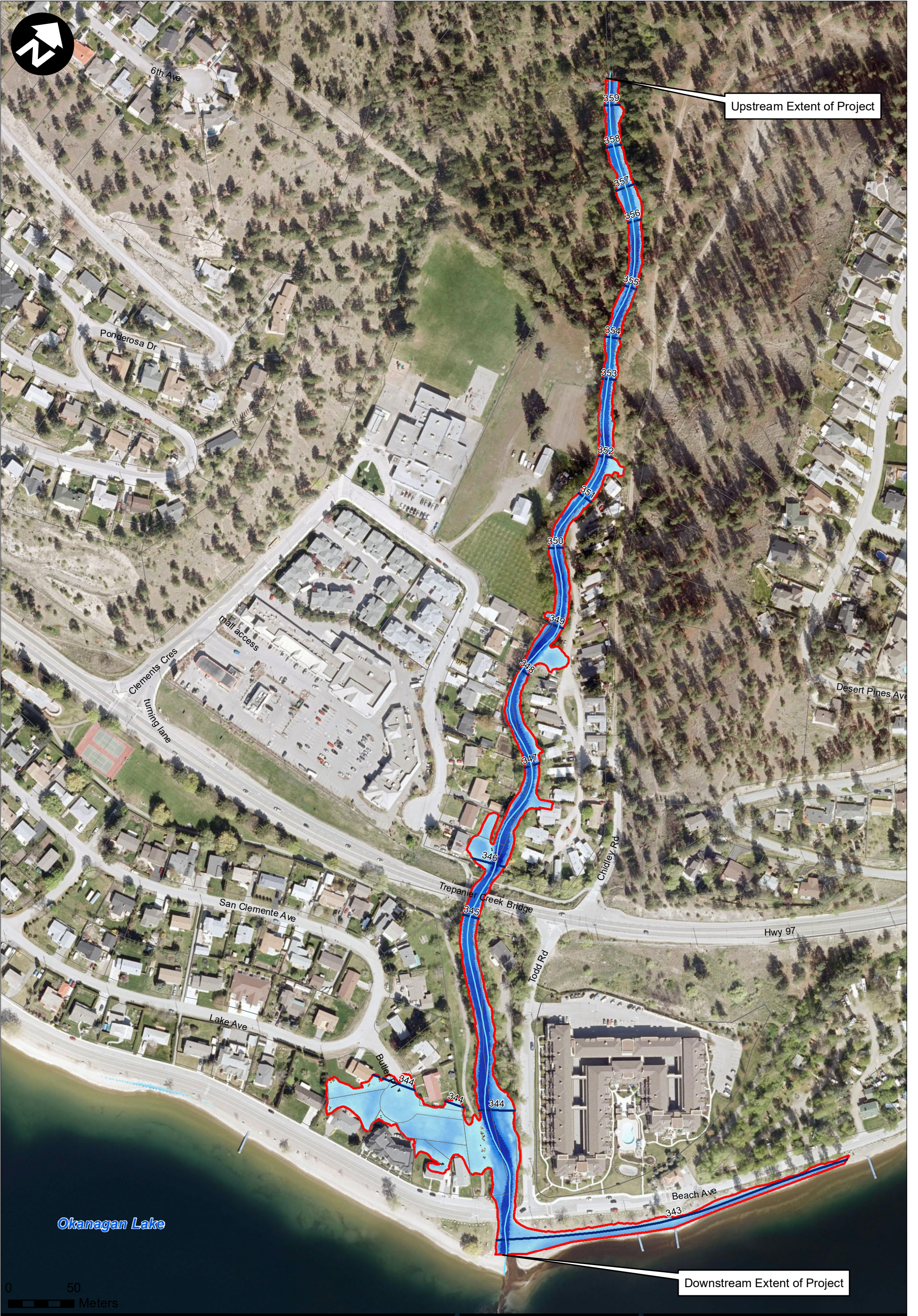
FIGURE 5-5: TREPANIER CREEK REACH 2, 20 YEAR - NO FREEBOARD RDCO Peachland and Trepanier Creeks Flood Mapping
