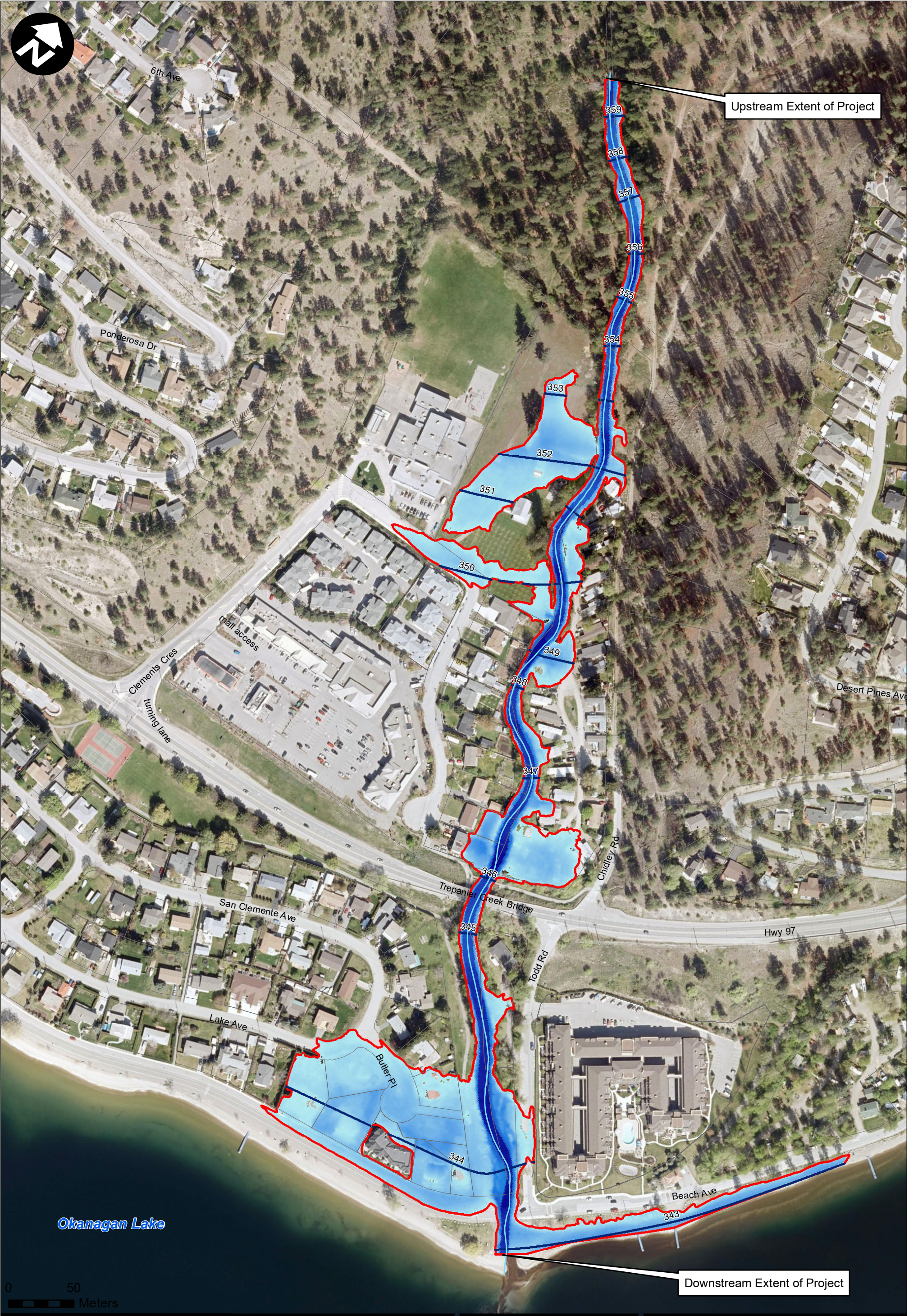
FIGURE 5-7: TREPANIER CREEK REACH 2, 200 YEAR - NO FREEBOARD RDCO Peachland and Trepanier Creeks Flood Mapping
