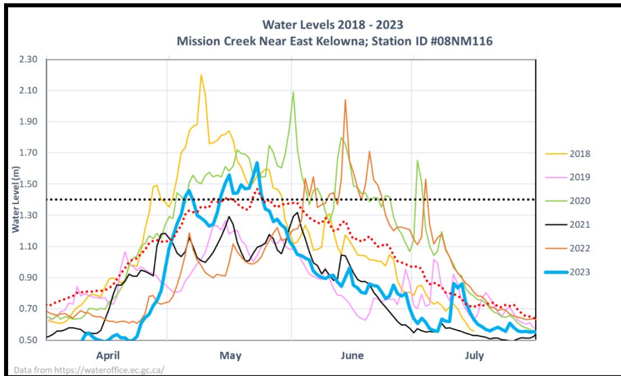
Figure 1: Mission Creek Levels, measured at East Kelowna (Station # 08NM116) 2018-2023.
