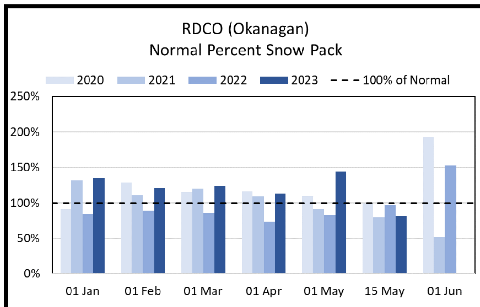
Chart 2: Snow Surveys; Percent of Normal Snowpack for 01 January – 01 June, 2020-2023, Okanagan Snow Basin ( www.bcrfc.gov.bc.ca )
