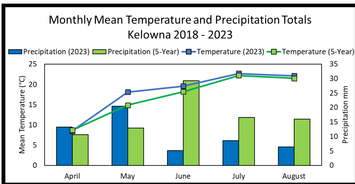
Chart 3: Monthly mean temperature and precipitation totals for April – August 2023 compared with the 2018-2022 averages. Measured at Kelowna UBCO, Station ID # 1123996
