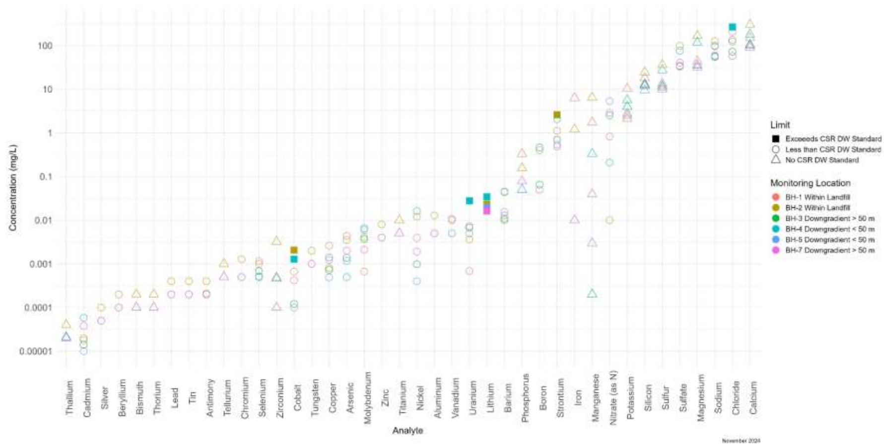
Figure 5: Groundwater Quality Summary, November 2024
