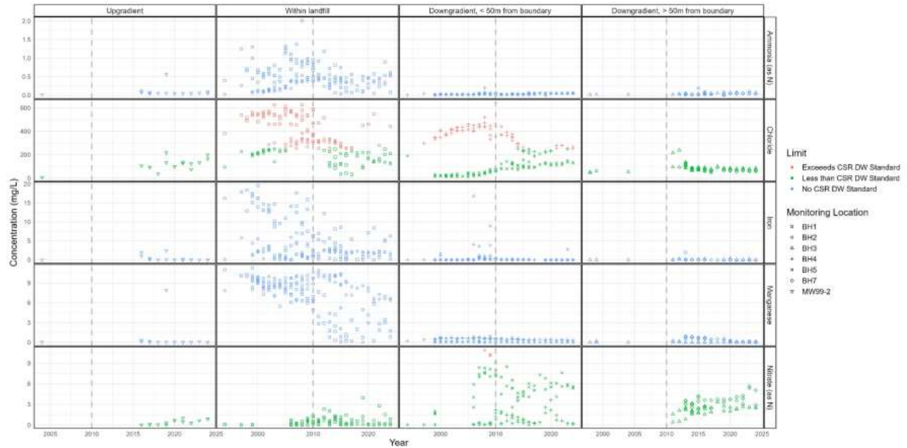
Figure 6: Concentrations of Key Parameters in Groundwater Over Time
