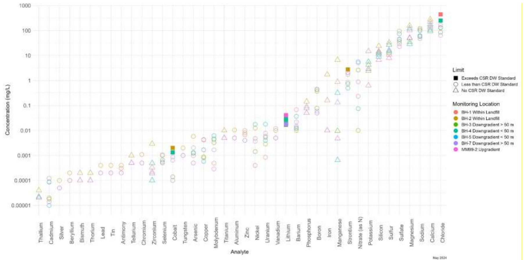
Figure 4: Groundwater Quality Summary, May 2024
